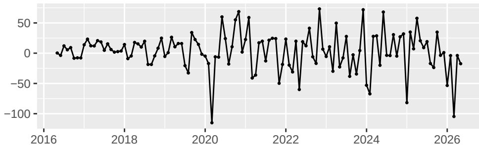
Residuals from ARIMA(0,1,1)
